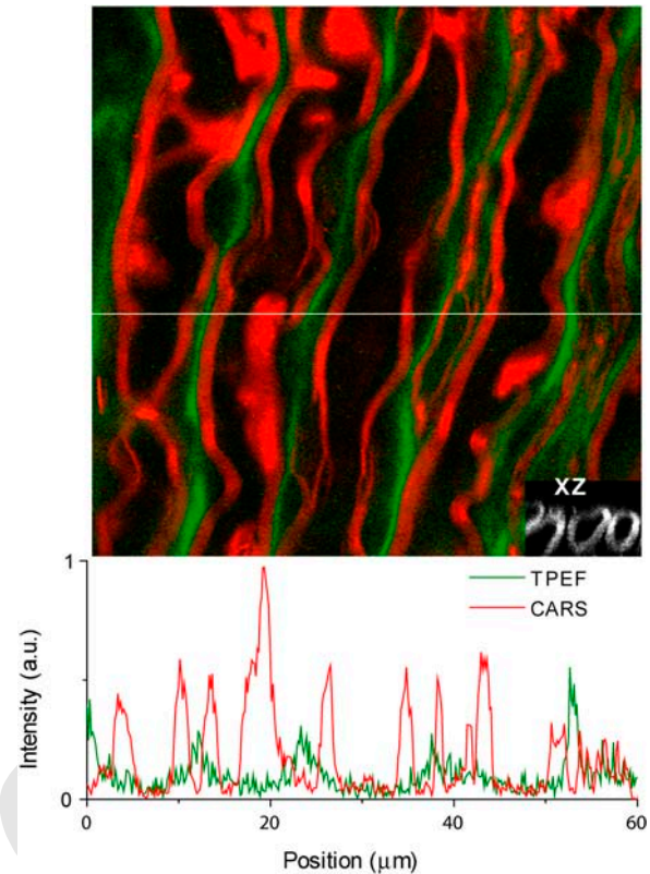
FIGURE 8 Simultaneous CARS imaging of axonal myelin and TPEF imaging of Oregon green 488. The pump and Stokes laser frequencies were tuned to 14,088 \text{ cm}^{-1} (710 nm) and 11,248 \text{ cm}^{-1} (889 nm), respectively. The E-CARS and TPEF signals are represented by the red and green colors, respectively. The intensity profiles along the white line are shown below the image. The grayscale inset image is an XZ image showing the cross section of axons. The 3D spatial resolution of CARS microscopy permits discrimination of the intraaxonal from extraaxonal space.
