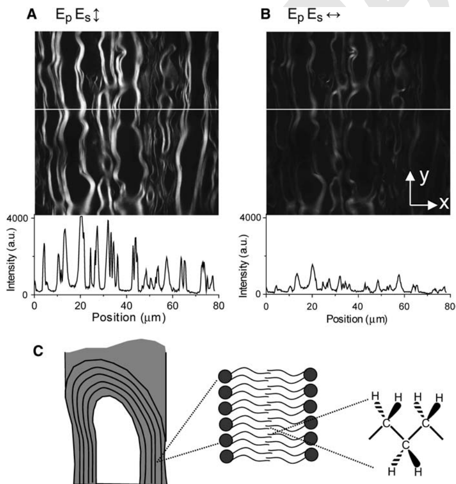
FIGURE 4 F-CARS images of myelin sheath using vertically polarized ( A ) and horizontally polarized ( B ) excitation beams. \omega_p - \omega_s was tuned to 2840 \text{ cm}^{-1} . The plots below the images are the intensity profiles for the lines shown in the images. ( C ) The symmetry axis of the \text{CH}_2 groups in the equatorial plane of the myelin is perpendicular to the x direction, leading to a larger I_{\parallel} than I_{\perp} .
